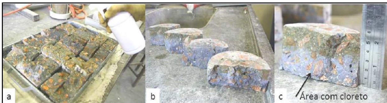
Figure 1. a) Spray silver nitrate solution; b) Comparison of the specimens; c) Measurement of the chloride penetration depth (MARCONDES, 2012)
