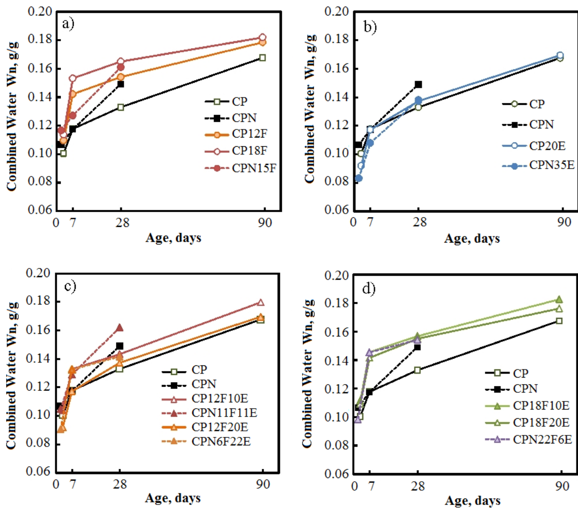
Figure 1: Evolution of the non-evaporable water (Wn) in the concrete matrix in function of time.
